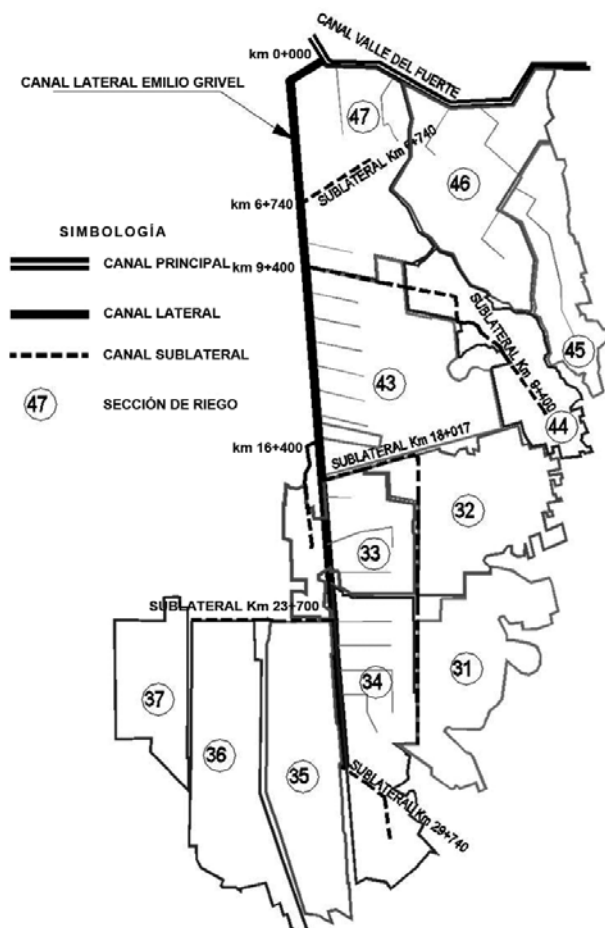
Figura 1. Plano del módulo de riego "Santa Rosa" del distrito de riego 075. Figure 1. General map of "Santa Rosa" irrigation zone at irrigation district 075.
