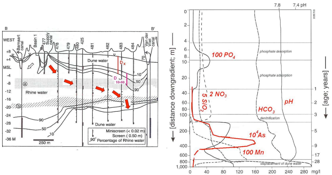
Figure 8.11 Site 6. Left: Position of the studied flow path of artificially recharge Rhine River water from the supply canal to the prograding intrusion front into deep dune groundwater. a = very fine, silty, marine Holocene sand (moderate aquitard); b = sandy, marine, Holocene clay (aquitard). Right: quality evolution anno 1981, along the flow path indicated in the cross section at the left (after Stuyfzand, 1993b).
