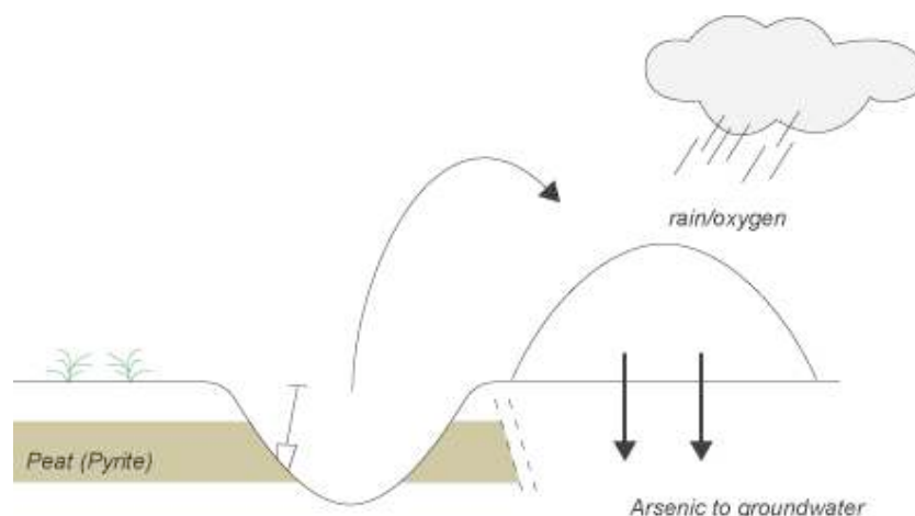
Figure 7.5 Effect of moving basal peat above the groundwater table.
