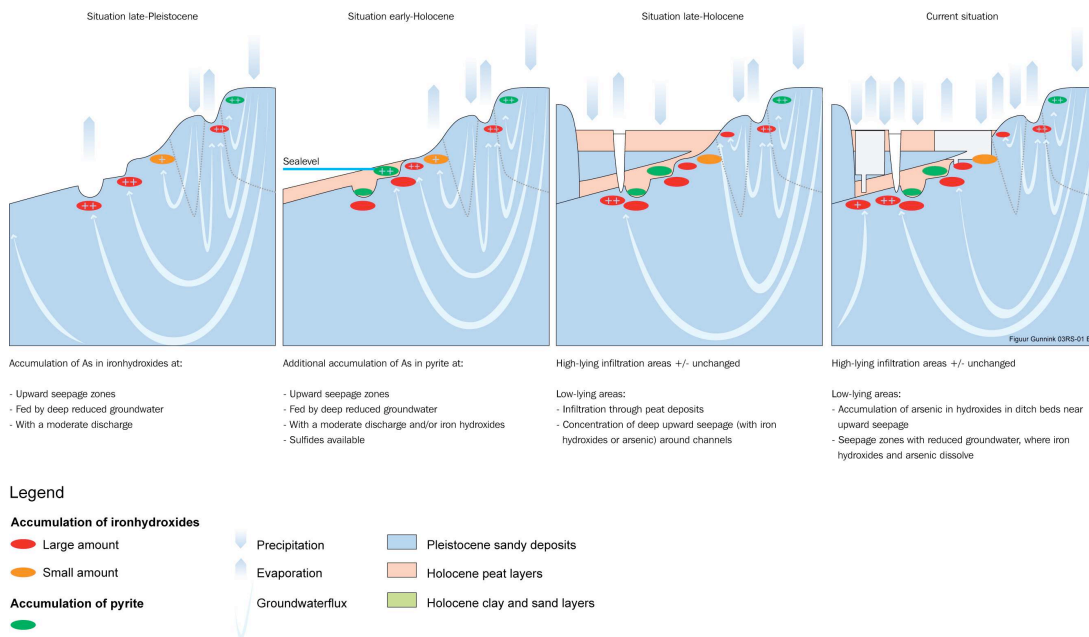
Figure 7.1 Processes causing high concentration of natural arsenic.
