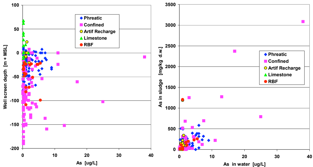
Figure 8.4 Plot of total dissolved As versus resp. depth of well screen in 1989, and As in sludge, for all well fields (for drinking water supply) in the Netherlands. Data from files Kiwa Water Research.
