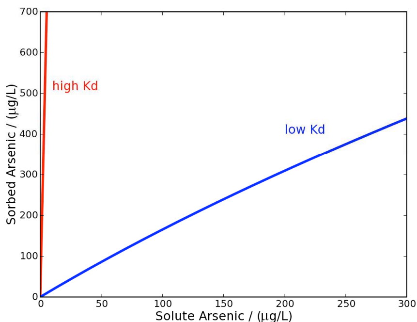
Figure 3.9 Calculated sorption isotherms for As in a Bangladesh aquifer. Curve “high Kd” is for 0.2 g ferrihydrite/L and with reduced surface complexation constants for \text{HCO}_3^- . Curve “low Kd” is for 10 times less ferrihydrite and 10 times higher surface complexation constants for \text{HCO}_3^- and has about 100 times smaller slope.
