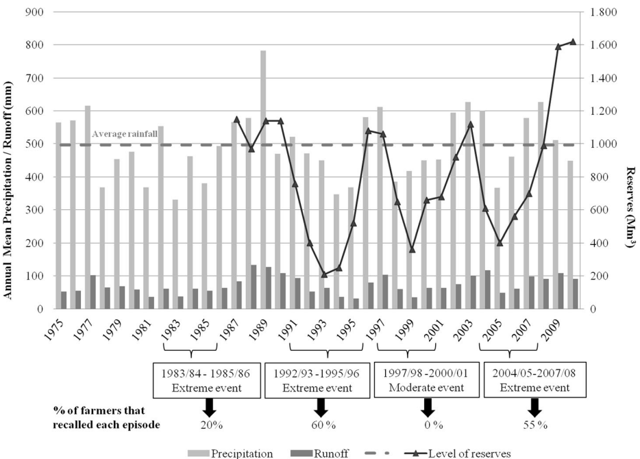
Fig. 3 Precipitation, runoff and surface water reserves in the JRBD
