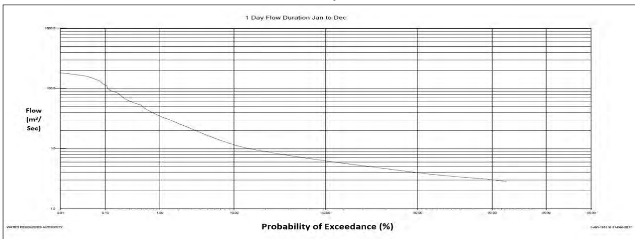
Figure 2. Flow Duration Curve of Mean Daily Stream Flow Exceedance Frequency from Rio Bueno at Rio Bueno station for January 1 st , 1951 to December 31 st , 2017
