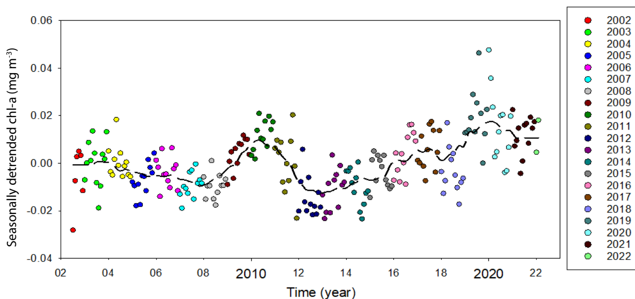
Figure 2.7. Seasonally detrended, global monthly mean values of oceanic chl-a from July 2002 to February 2022 [colour coded by year] with a running average [dashed line]. Source: Analysis based on data obtained via the Giovanni online data system, developed and maintained by the NASA GES DISC.
