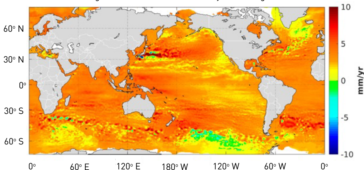
Regional sea level trends (January 1993 - August 2021)
