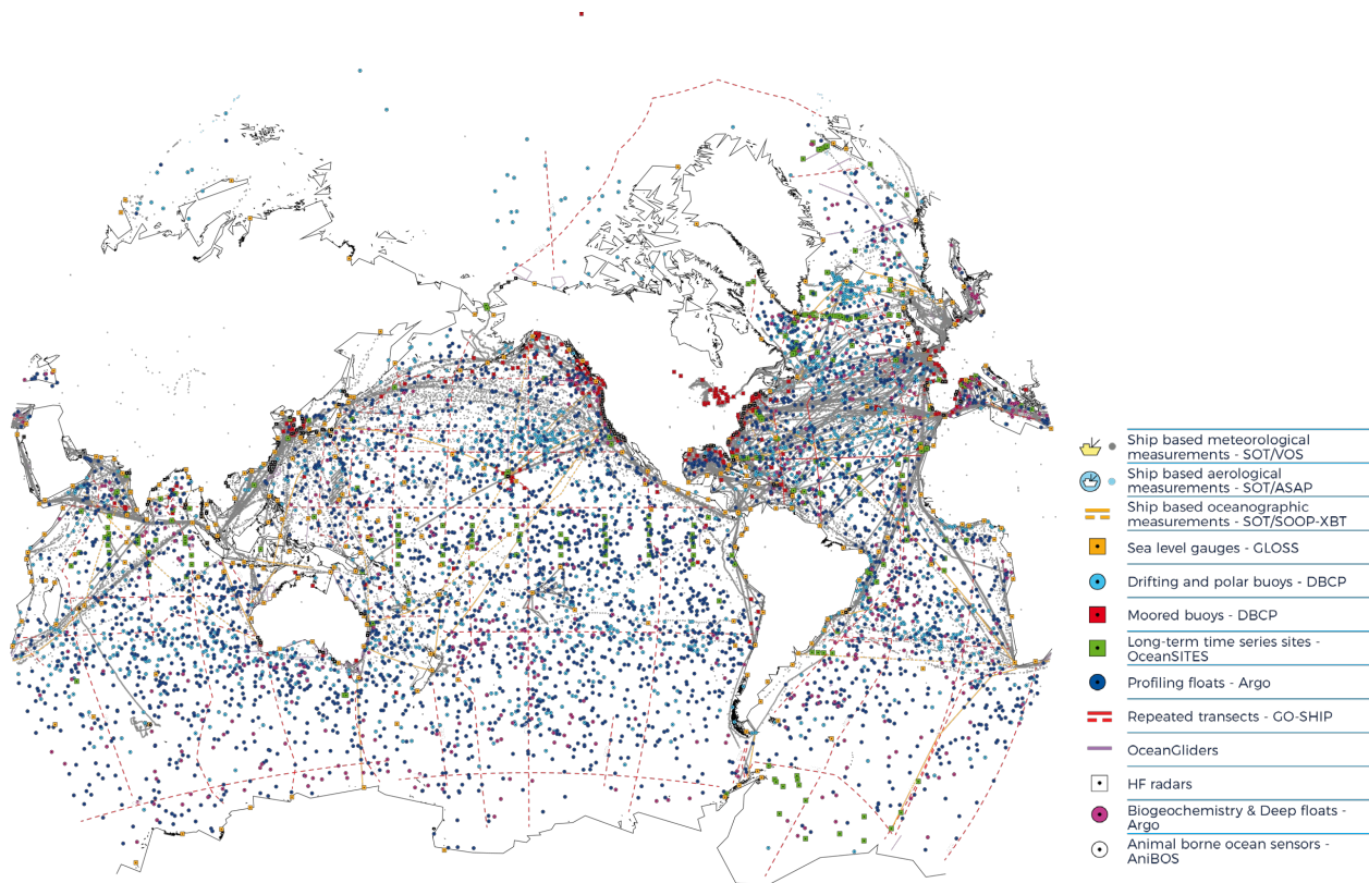
Figure 7.1. In situ Global Ocean Observing System.
