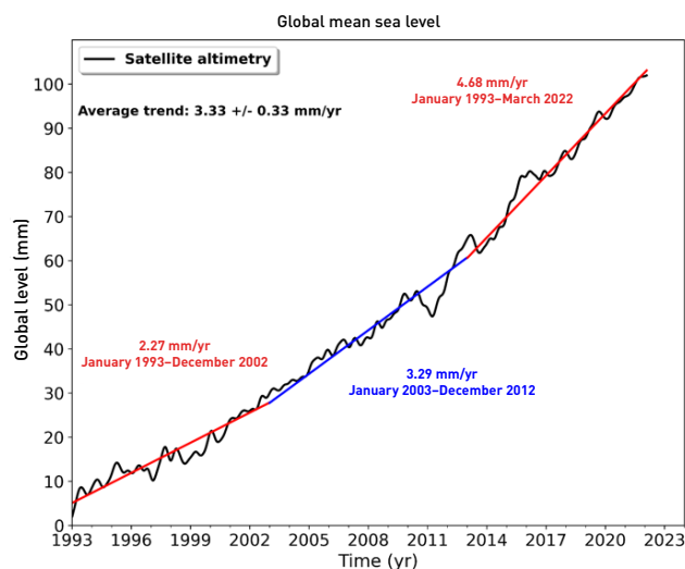
Figure 6.2. Global mean sea level rise from satellite altimetry from January 1993 to March 2022 (black curve). The red and blue straight lines indicate successive global mean sea level trends. Altimetry data from AVISO https://www.aviso.altimetry.fr Source: Cazenave and Moreira, 2022.
