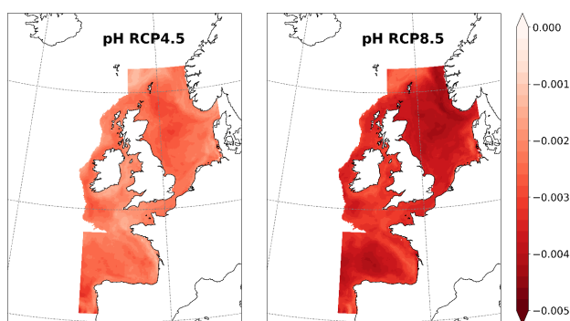
Figure 2.4. Trend of surface pH ( \text{yr}^{-1} ) between 2000 and 2050 as projected by the AMM7-NEMO-ERSEM model under the RCP 4.5 scenario (left) and RCP8.5 scenario (right). Only data within the OSPAR regions has been shown. Source: OSPAR QSR2023 OA Assessment, in press.
