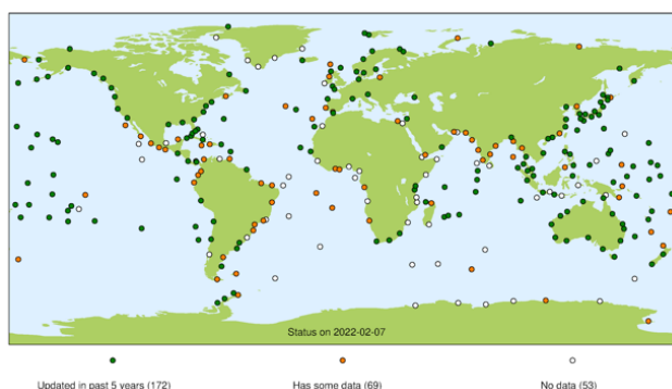
Figure 6.4. Current status of the in situ GLOSS core network of tide gauges at the Permanent Service for Mean Sea Level (PSMSL). Source: Holgate et al., 2013.
