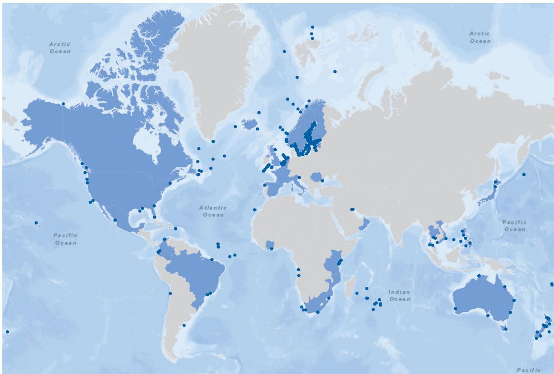
Figure 2.1. Map illustrating surface ocean carbonate chemistry measurement locations received for 14.3.1 ocean acidification reporting: countries which submitted data are colored in blue and dots indicate the location of measurements.
