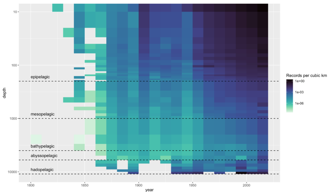
Figure 8.2. The number of records in OBIS per volume ( \text{km}^3 ) by depth and by year (produced on 23 Feb 2022). Source: OBIS.
