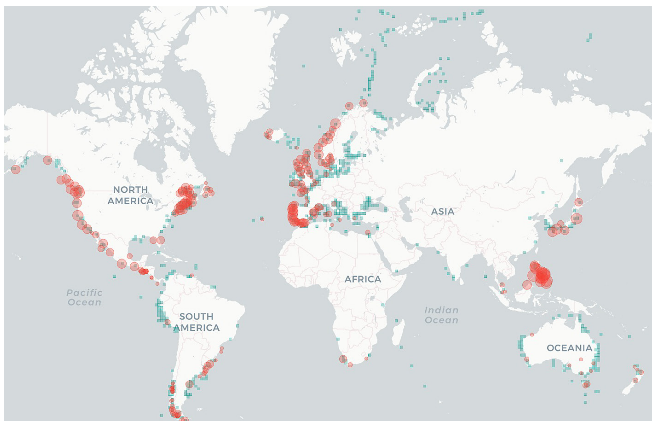
Figure 6.8. World map of distribution events associated with paralytic shellfish toxins (red) combined with that of the occurrence of Alexandrium causative organisms (blue). Source: based on data obtained from the HAIS Data Portal https://data.hais.ioc-unesco.org/ .
