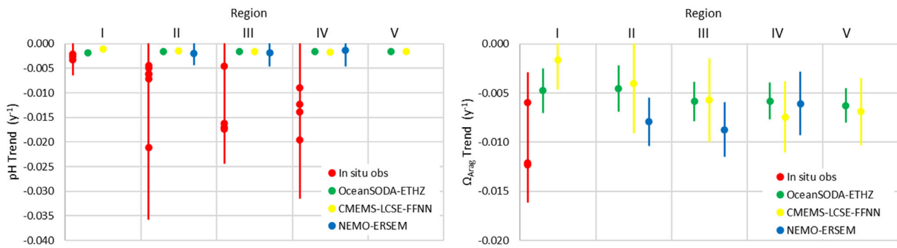
Figure 2.3. Overview on trends in pH (left panel) and aragonite saturation state ( \Omega_{Arag} ; right panel) for each of the OSPAR regions (I = Arctic Waters; II = The Greater North Sea; III = The Celtic Seas; IV = Bay of Biscay and Iberian Coast; V = Wider Atlantic) using different data types (in situ observation time-series stations [red], reconstruction synthesis products: OceanSODA-ETHZ (green) and CMEMS-LCSE-FFNN (yellow), and modelling: NEMO-ERSEM (blue)). Trends are only included if they are statistically significant, and for time-series stations only if the station has data for more than 10 years. Note the reconstruction and modelling products are regionally weighted average (mean) trends. Error bars represent standard deviation around the trend. Source: OSPAR QSR2023 OA Assessment, in press.
