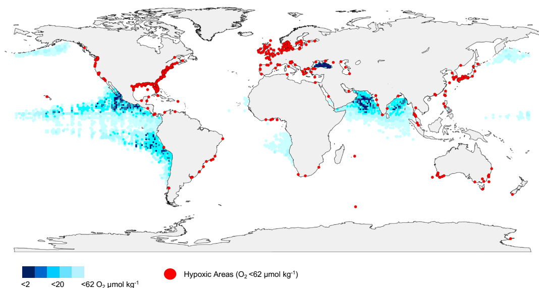
Figure 1.1. Locations of low O_2 areas (i.e. O_2 < 62 \mu\text{mol kg}^{-1} ) in the coastal and global ocean. In the coastal zone, more than 500 sites have been inventoried with low O_2 conditions in the past half century (red dots); in the open ocean O_2 waters encompass several million \text{km}^3 (blue dots refer to conditions at 300 m depth). Source: Adapted from Breitburg et al., 2018.
