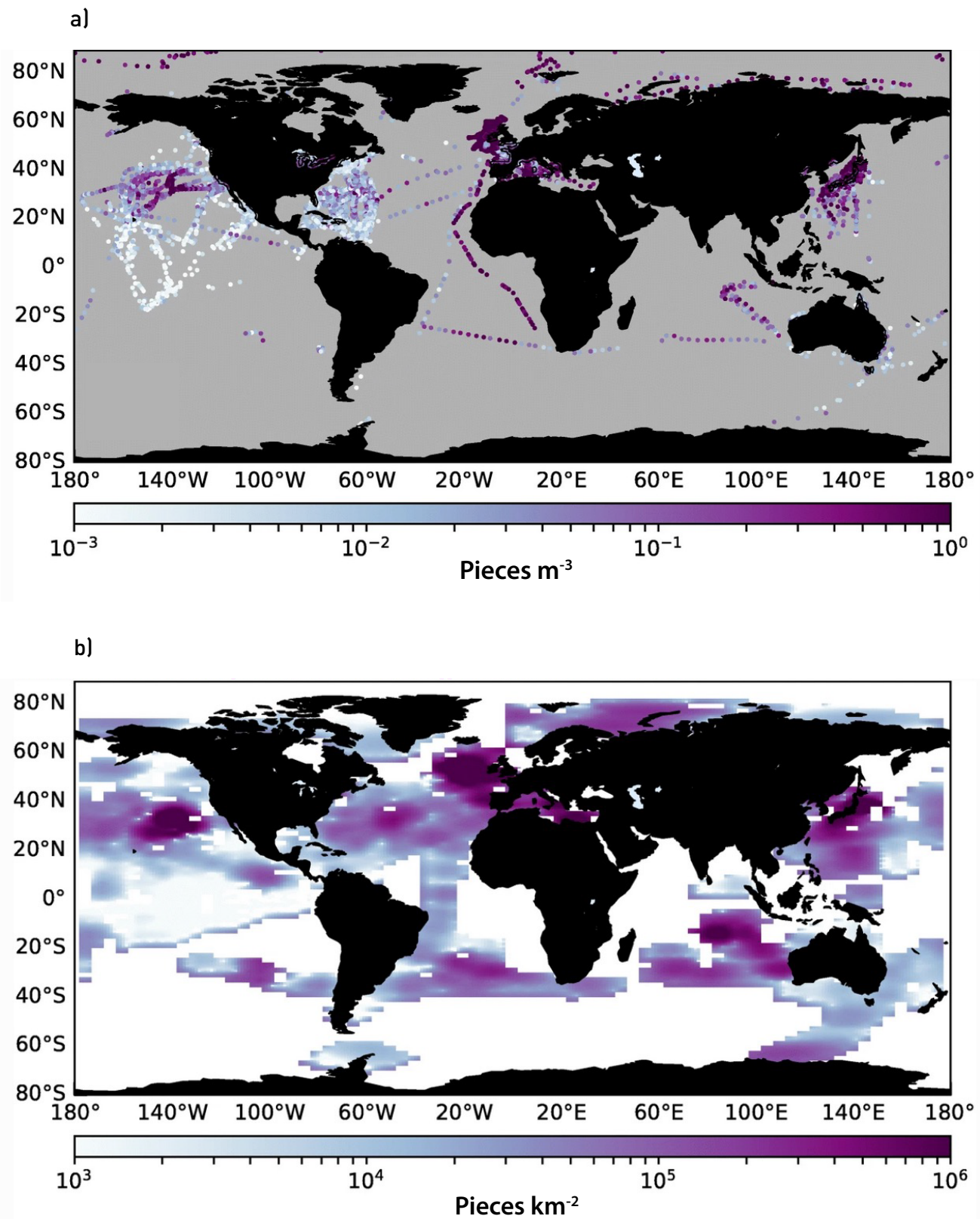
Figure 1.4. Abundance of microplastics in the world's upper ocean and the Laurentian Great Lakes, based on 8,218 microplastic samples. a) abundance showing sampling locations; b) gridded data based on an optimum interpolation method which yields an estimated 24.4 trillion pieces ( 8.2 \times 10^4 – 57.8 \times 10^4 tonnes). Source: Isobe et al., 2021.
