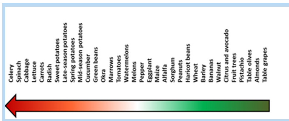
Figure 5.5. Increasing potential of CEC uptake by different plant species
