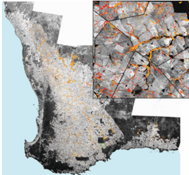
Figure 3. Example of dryland salinity mapping in Western Australia: multi-temporal change detection with 10m DEM and ground truth (GPS, vegetation cover, soil condition). The subregion covers 16 x 16 km: areas mapped as salt affected in 1988 are orange, with additional areas in red in 1998.
